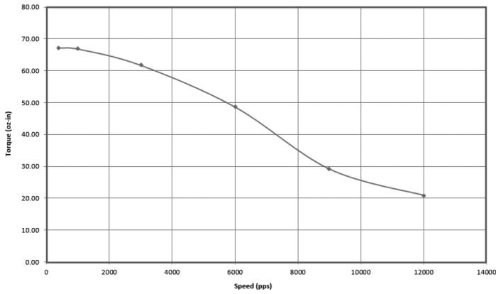
CUI Devices P/N NEMA23-17-01SD-AMT112S Lin Engineering P/N WD-5718X-01S (1.8 Step Motor) 24 Vdc, 1.4 Amp/Phase, Bipolar, 1/2 Stepping
