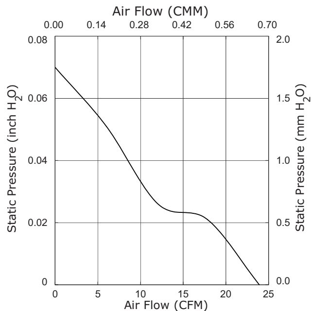
CFM-8025V-120-204
