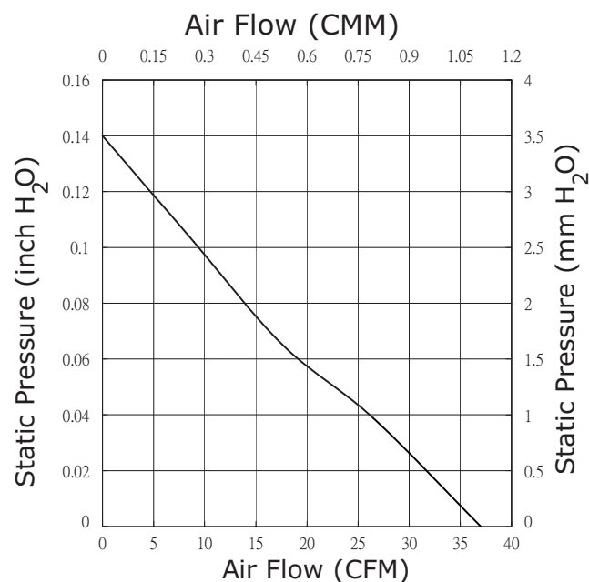
CFM-8020V-130-350
