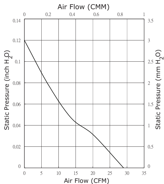
CFM-8020V-226-300
