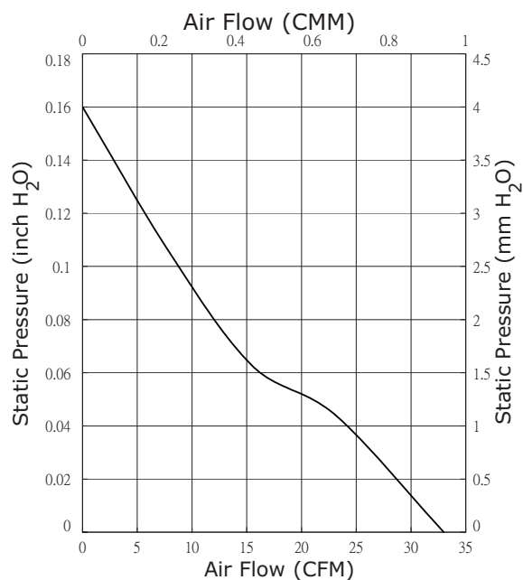
CFM-8020V-230-350
